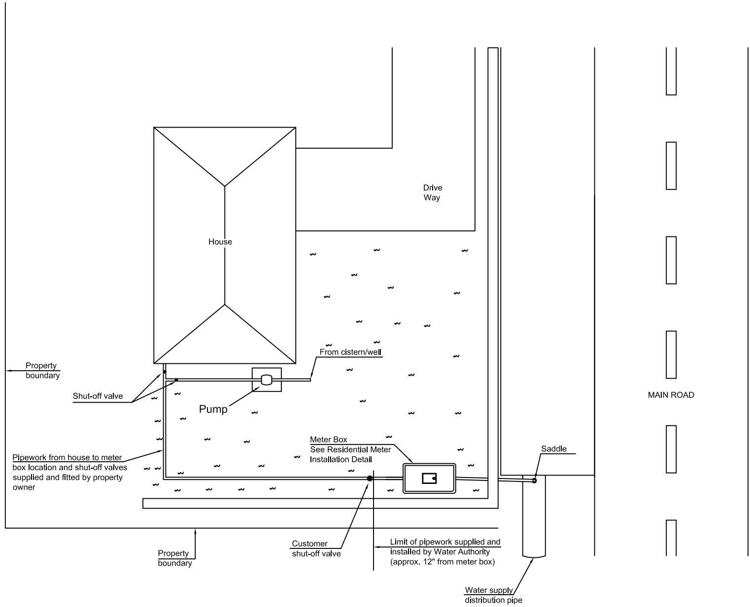
Water Authority - Cayman Typical Residential Connection To Main Water Supply Plan View
