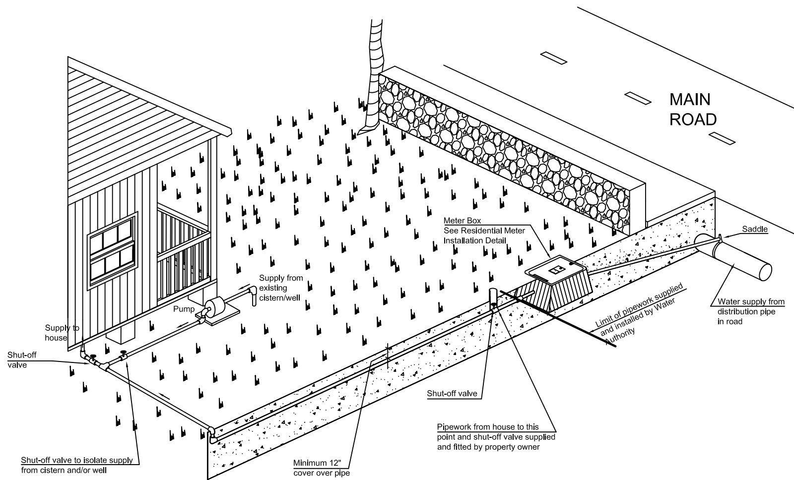
Water Authority - Cayman Typical Residential Connection To Main Water Supply Isometric View
