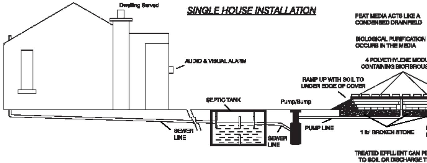
Figure 2. Fixed film system using peat moss as a treatment medium
